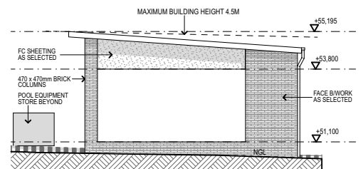
NORTH ELEVATION
