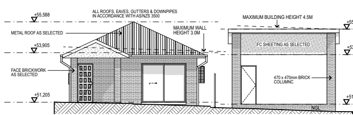
EAST ELEVATION
