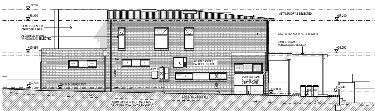
NORTH ELEVATION
